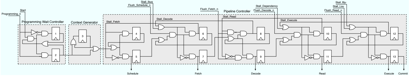
Figure 8: Generated circuit for the JackKnife pipeline controller.
